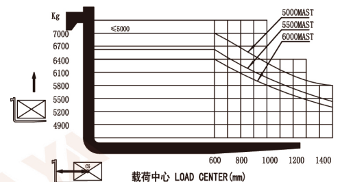
7.0T载荷曲线图 7.0T load curve
