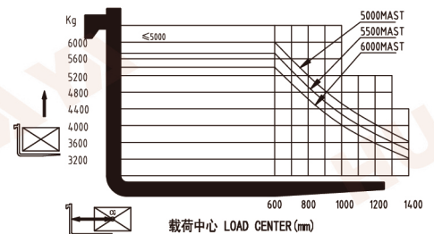
6.0T载荷曲线图 6.0T load curve
